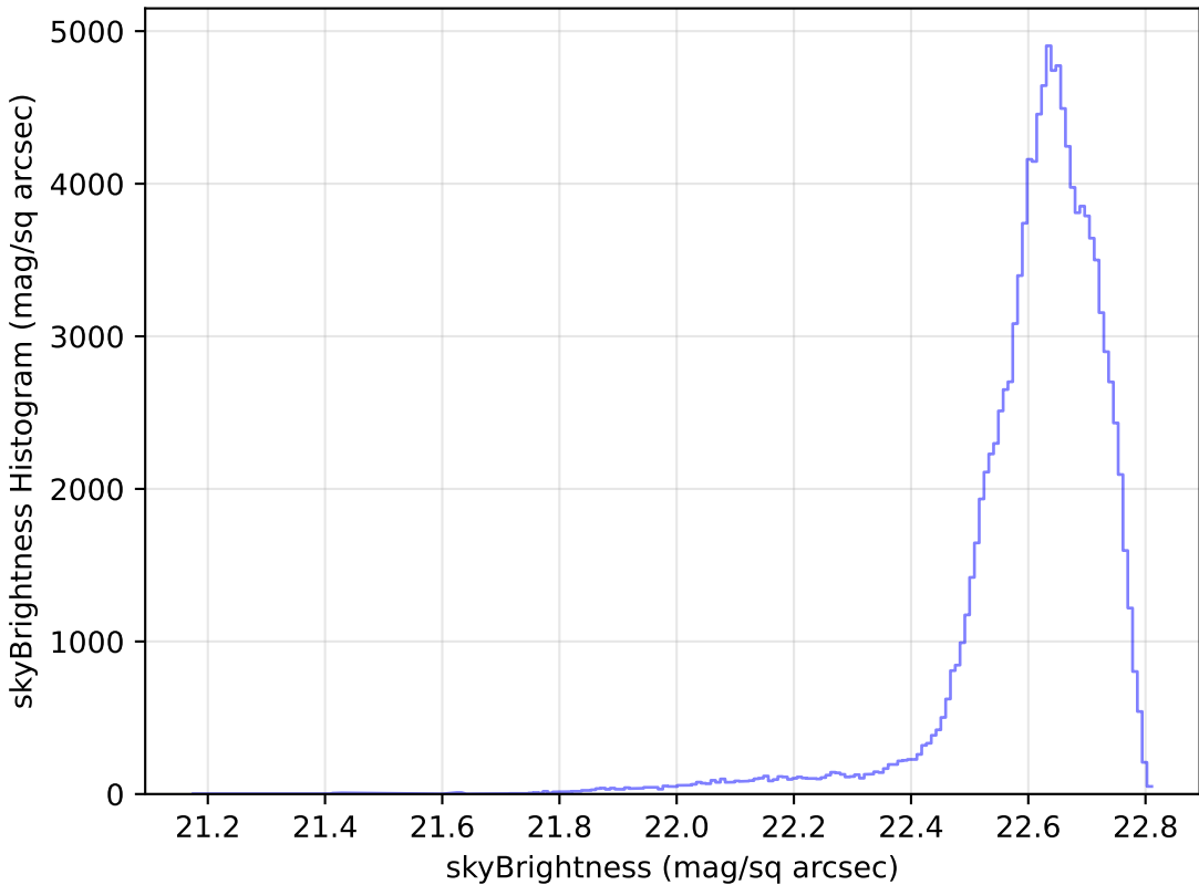
baseline_v3.3_10yrs All sky u band: skyBrightness Histogram
