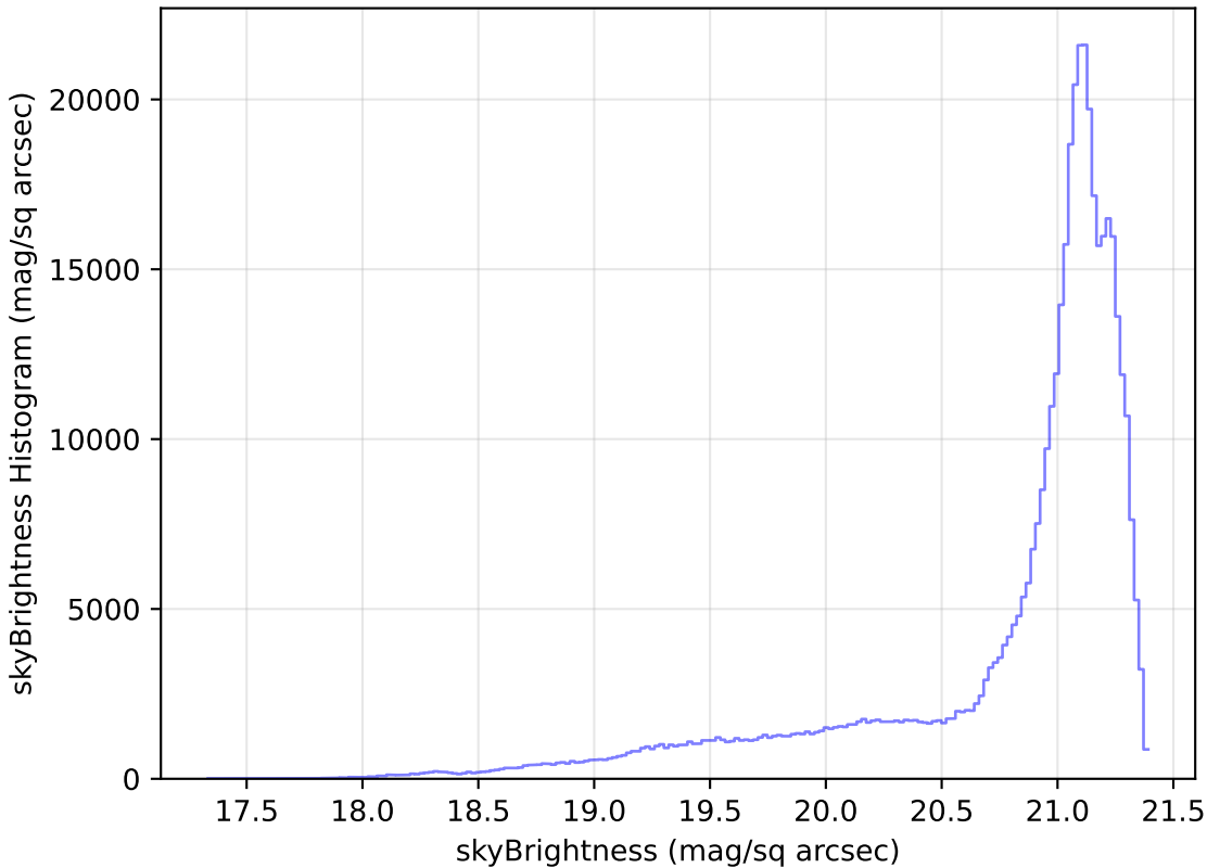
baseline_v3.3_10yrs All sky r band: skyBrightness Histogram
