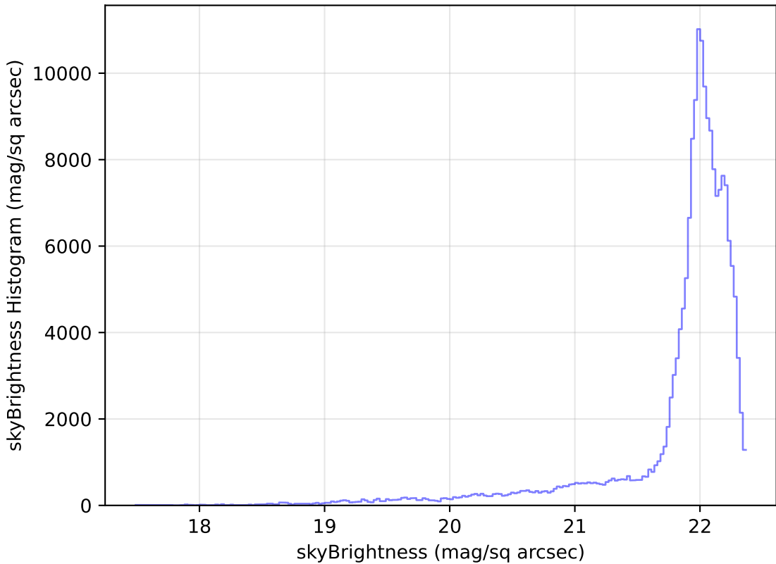
baseline_v3.3_10yrs All sky g band: skyBrightness Histogram
