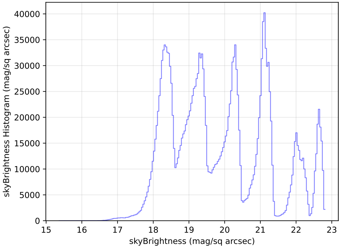
baseline_v3.3_10yrs All sky all bands: skyBrightness Histogram
