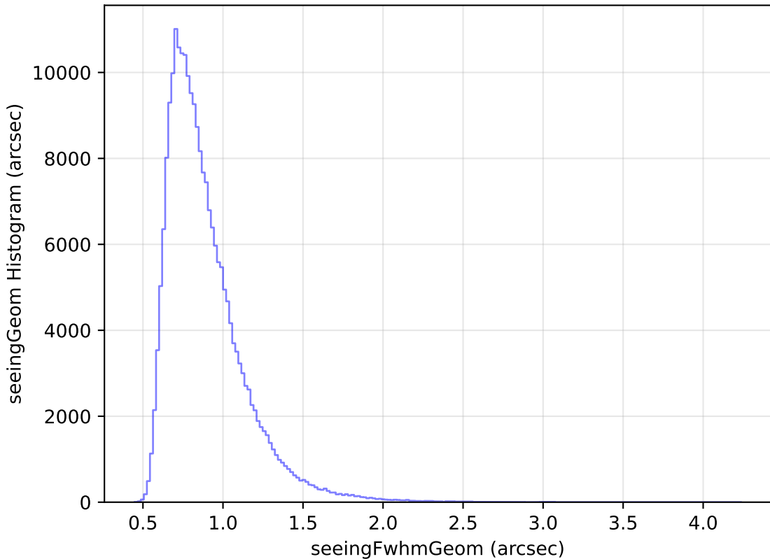
baseline_v3.3_10yrs Yr 1 all bands: seeingGeom Histogram
