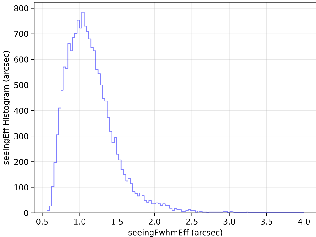
baseline_v3.3_10yrs Yr 1 u band: seeingEff Histogram
