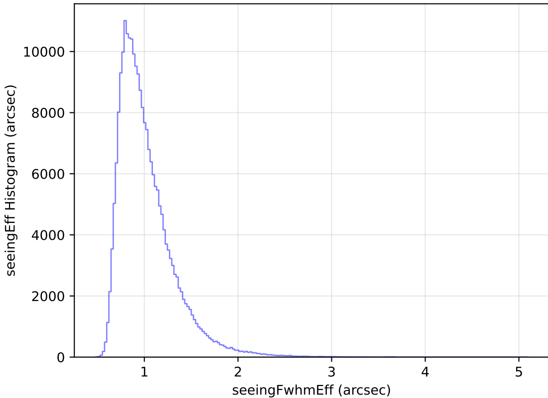
baseline_v3.3_10yrs Yr 1 all bands: seeingEff Histogram
