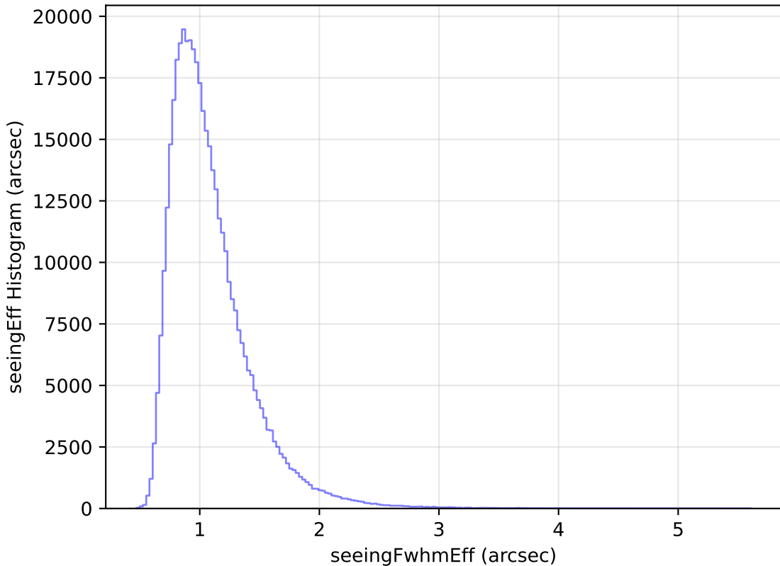
baseline_v3.3_10yrs WFD z band: seeingEff Histogram
