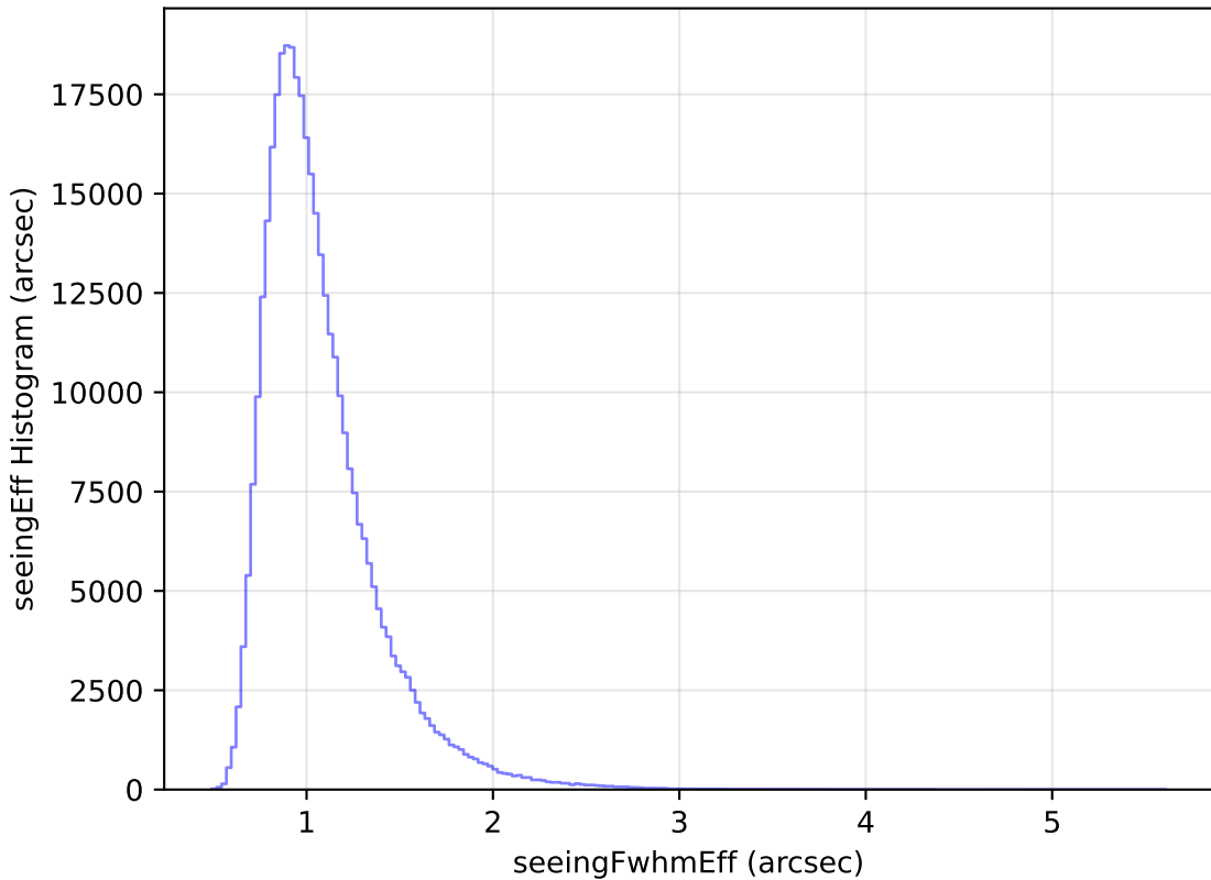
baseline_v3.3_10yrs WFD y band: seeingEff Histogram
