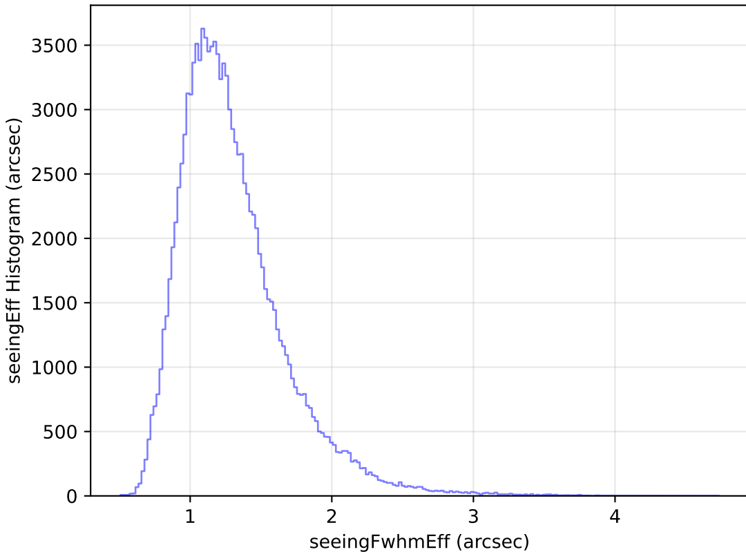
baseline_v3.3_10yrs WFD u band: seeingEff Histogram
