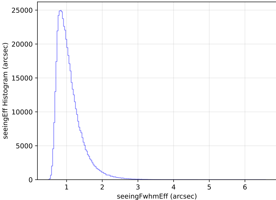
baseline_v3.3_10yrs WFD i band: seeingEff Histogram
