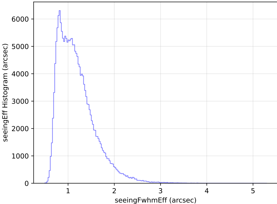
baseline_v3.3_10yrs WFD g band: seeingEff Histogram
