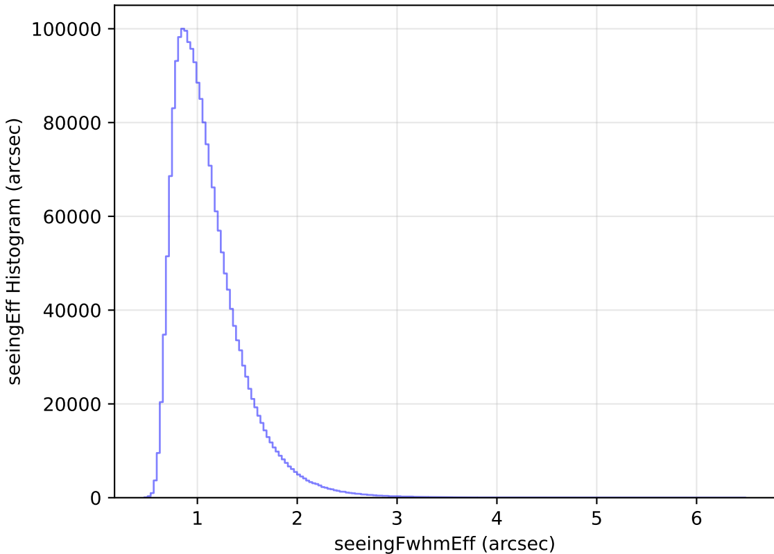
baseline_v3.3_10yrs WFD all bands: seeingEff Histogram
