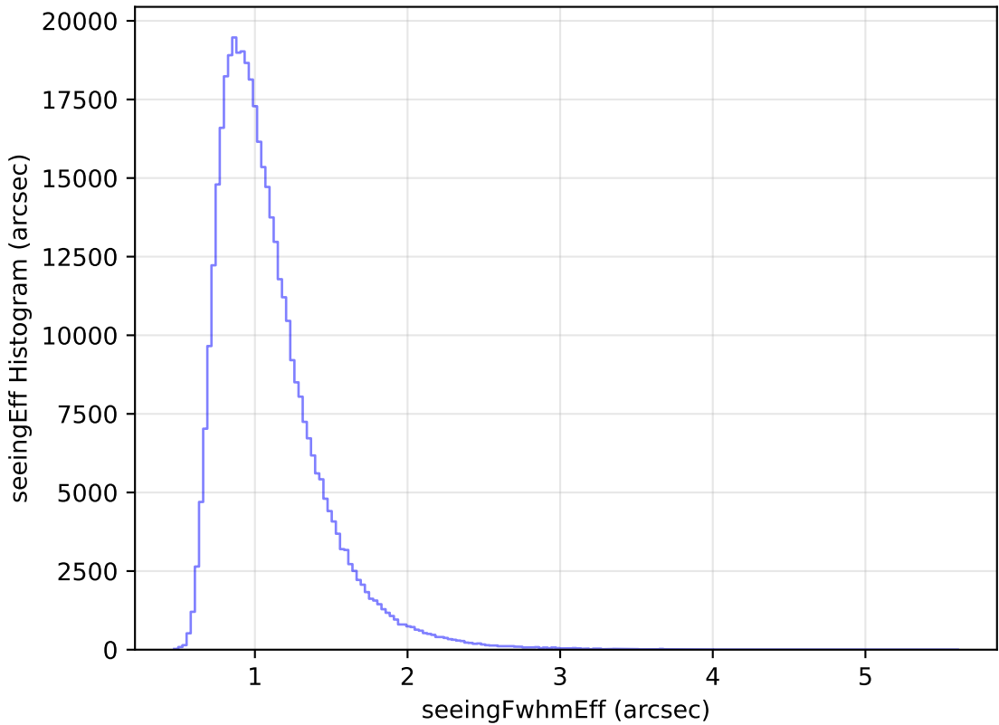
baseline_v3.3_10yrs All sky z band: seeingEff Histogram
