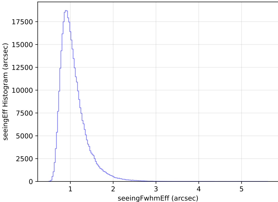
baseline_v3.3_10yrs All sky y band: seeingEff Histogram
