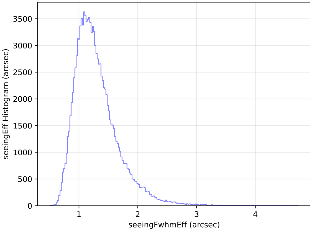
baseline_v3.3_10yrs All sky u band: seeingEff Histogram
