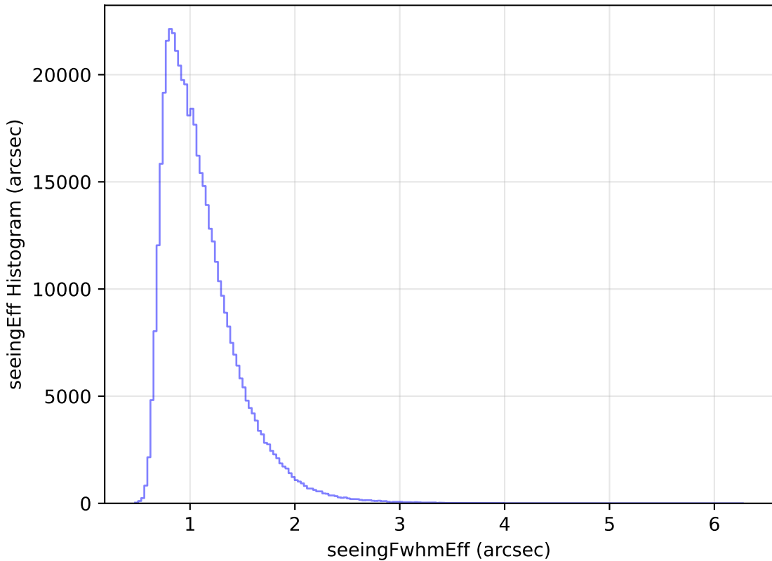
baseline_v3.3_10yrs All sky r band: seeingEff Histogram
