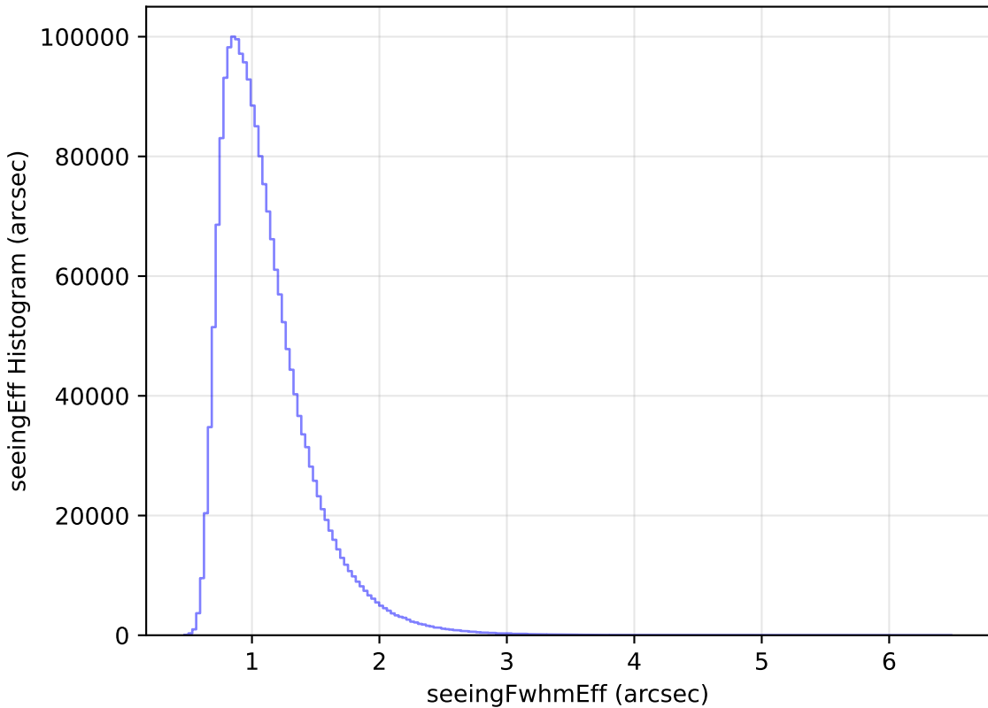
baseline_v3.3_10yrs All sky all bands: seeingEff Histogram
