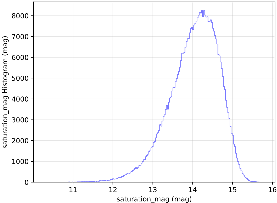
baseline_v3.3_10yrs WFD z band: saturation_mag Histogram
