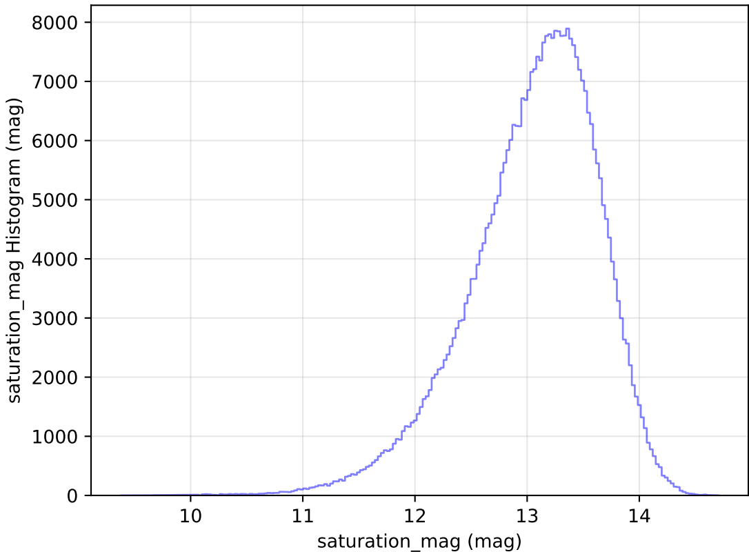
baseline_v3.3_10yrs WFD y band: saturation_mag Histogram
