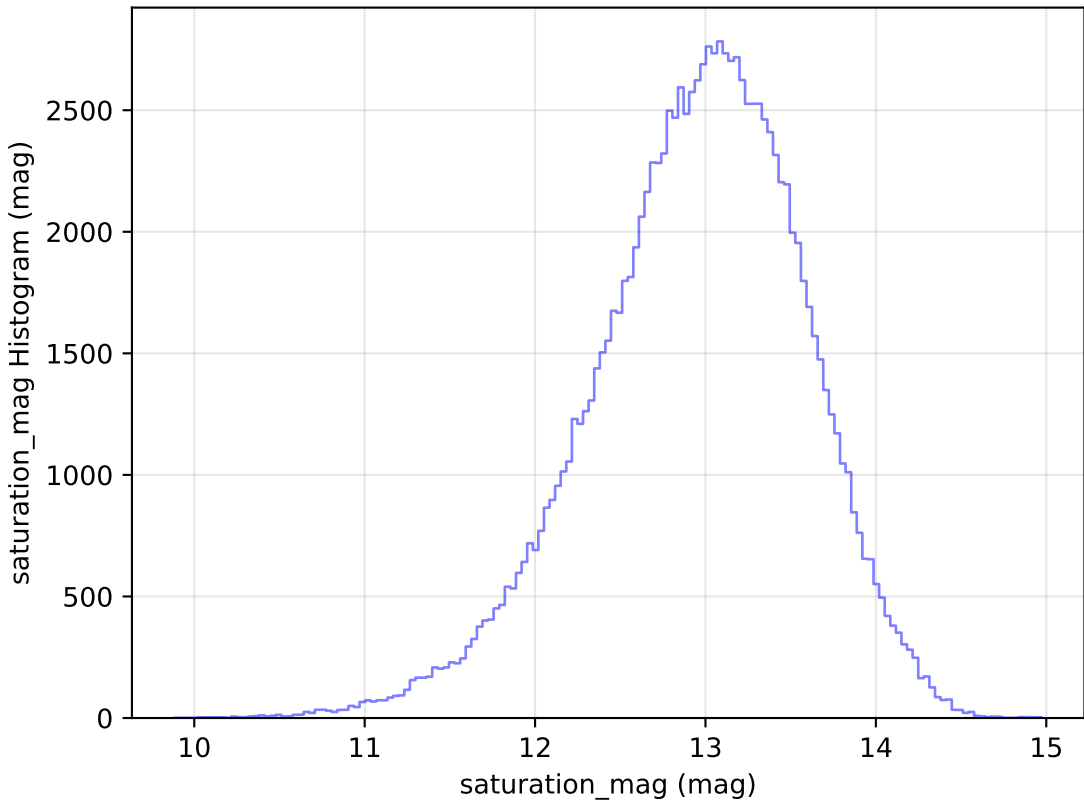
baseline_v3.3_10yrs WFD u band: saturation_mag Histogram
