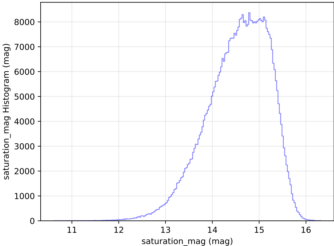
baseline_v3.3_10yrs WFD r band: saturation_mag Histogram
