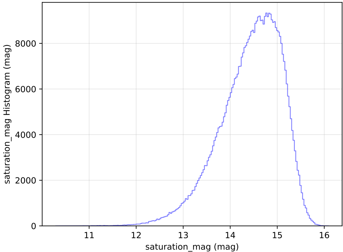
baseline_v3.3_10yrs WFD i band: saturation_mag Histogram
