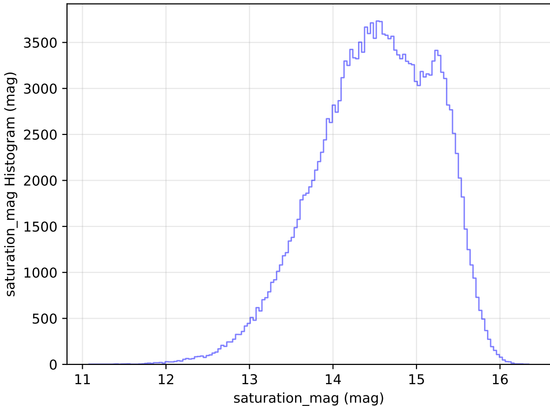
baseline_v3.3_10yrs WFD g band: saturation_mag Histogram
