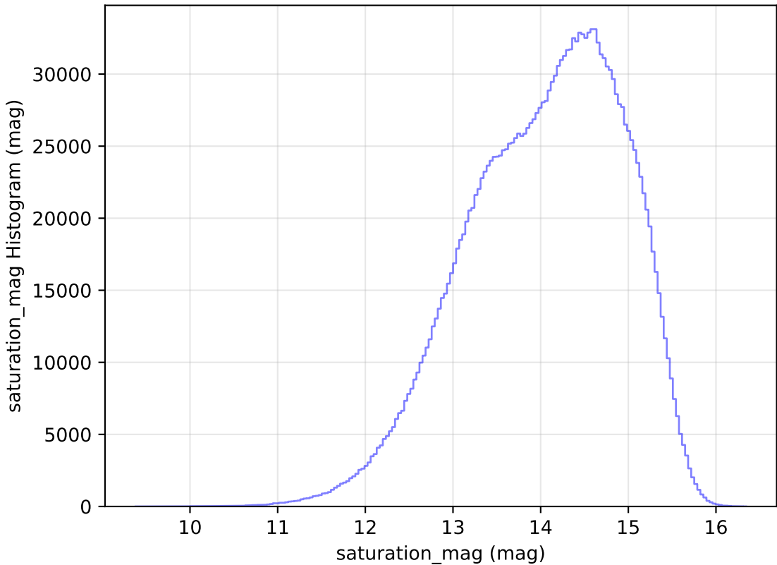
baseline_v3.3_10yrs WFD all bands: saturation_mag Histogram
