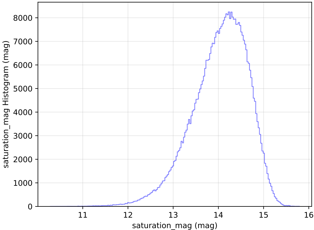
baseline_v3.3_10yrs All sky z band: saturation_mag Histogram
