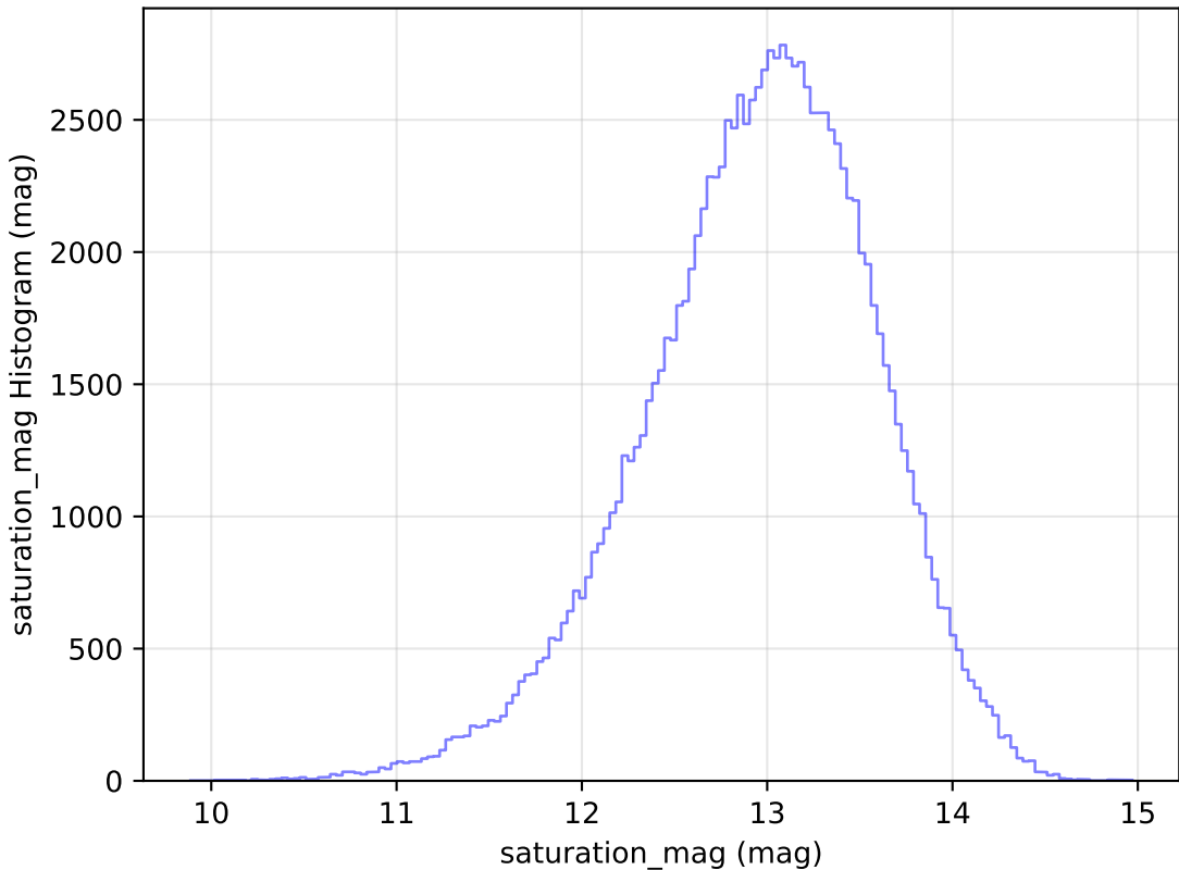
baseline_v3.3_10yrs All sky u band: saturation_mag Histogram
