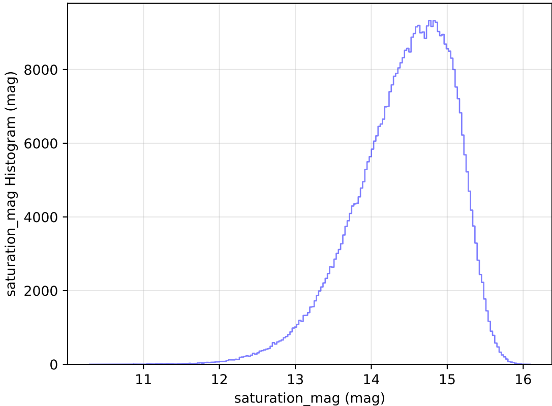
baseline_v3.3_10yrs All sky i band: saturation_mag Histogram
