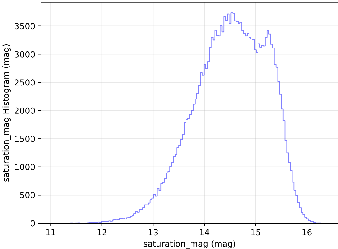
baseline_v3.3_10yrs All sky g band: saturation_mag Histogram
