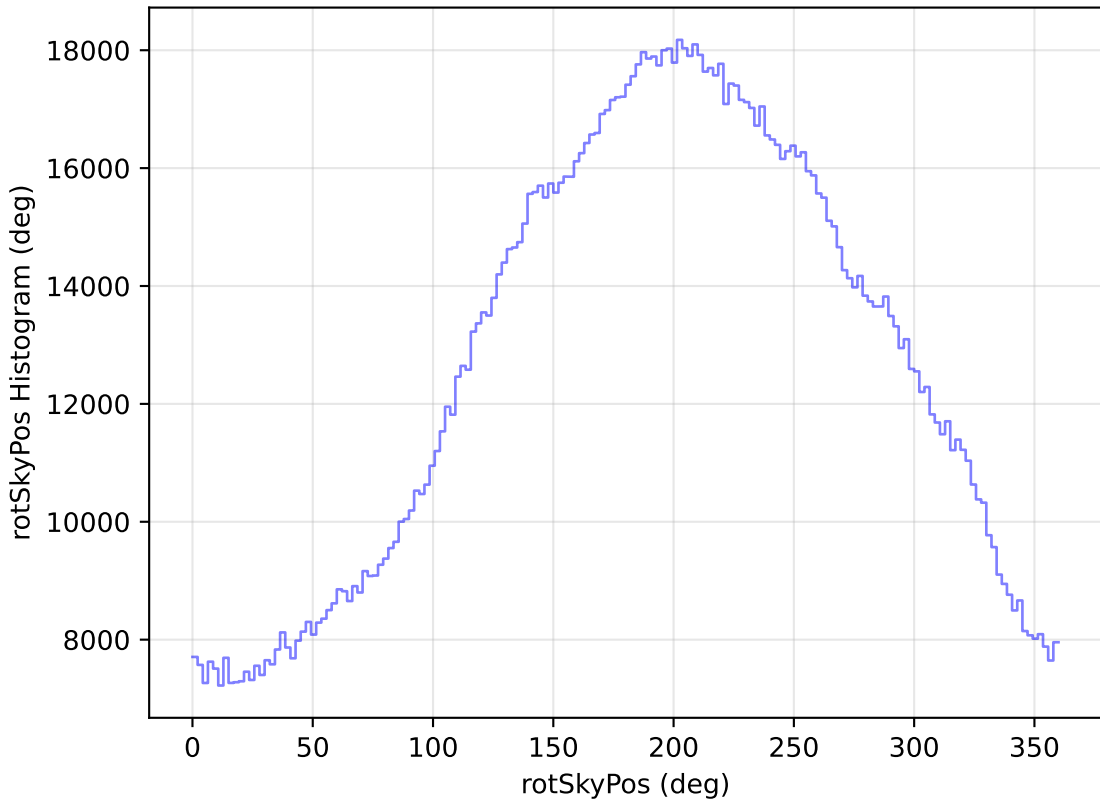
baseline_v3.3_10yrs WFD all bands: rotSkyPos Histogram
