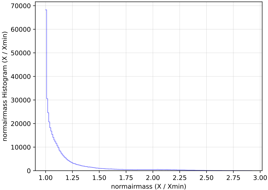
baseline_v3.3_10yrs WFD z band: normairmass Histogram
