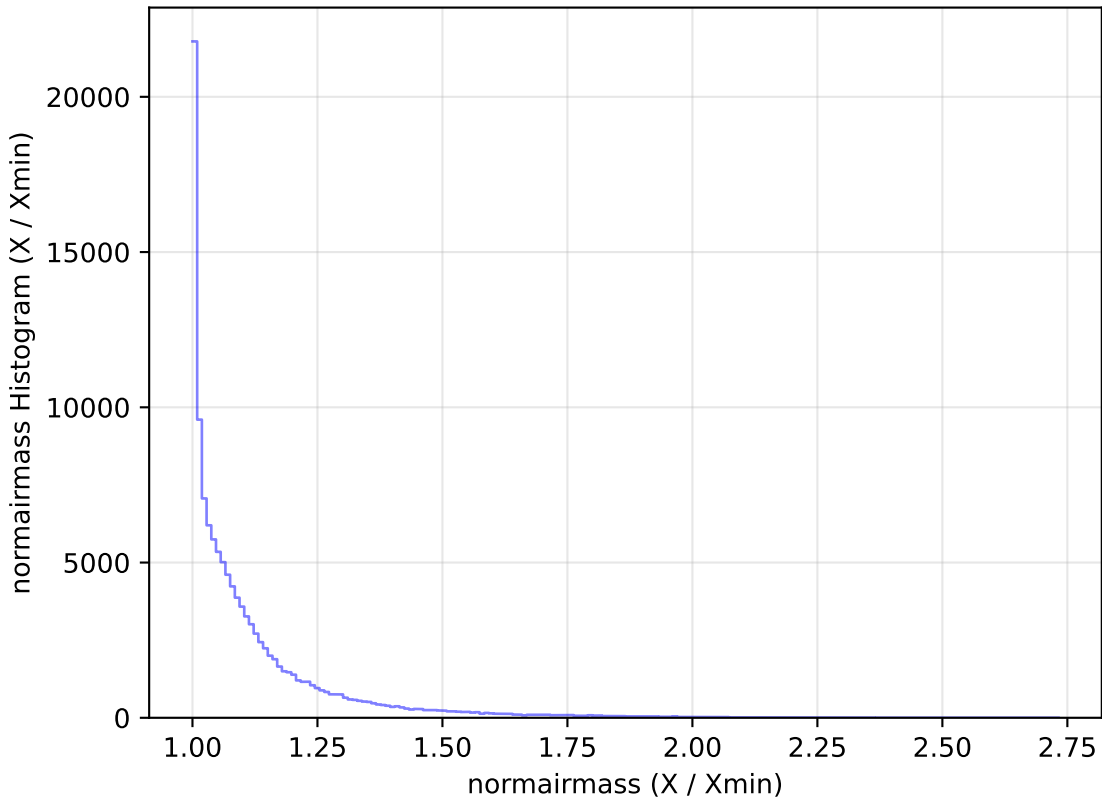
baseline_v3.3_10yrs WFD u band: normairmass Histogram
