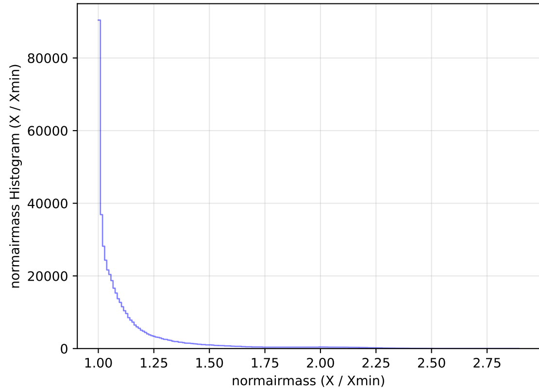
baseline_v3.3_10yrs WFD r band: normairmass Histogram
