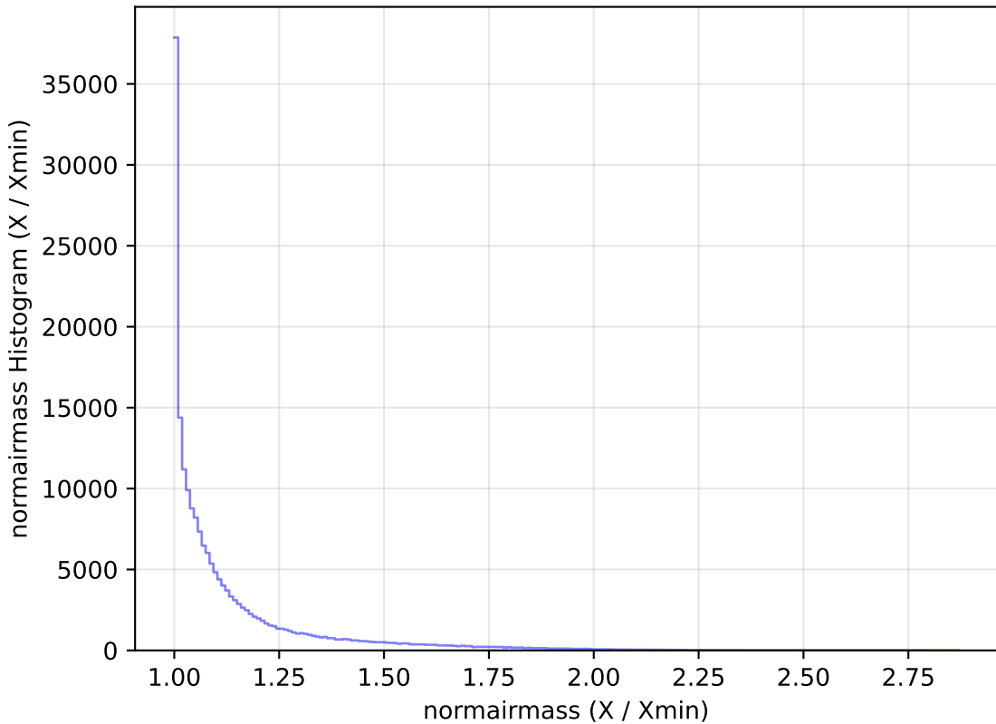
baseline_v3.3_10yrs WFD g band: normairmass Histogram
