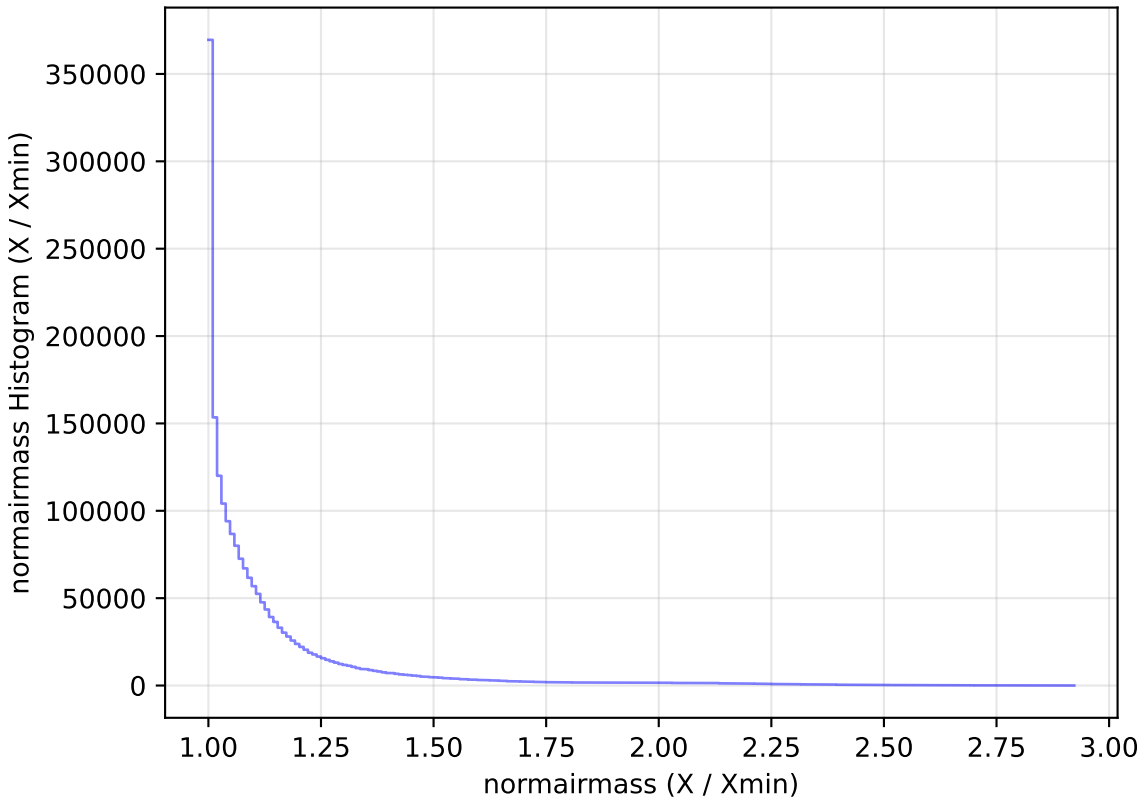
baseline_v3.3_10yrs WFD all bands: normairmass Histogram
