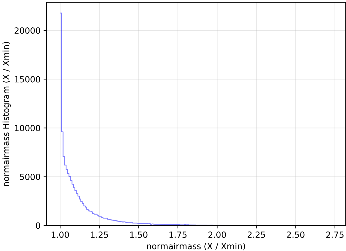
baseline_v3.3_10yrs All sky u band: normairmass Histogram
