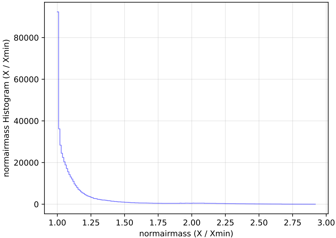
baseline_v3.3_10yrs All sky i band: normairmass Histogram
