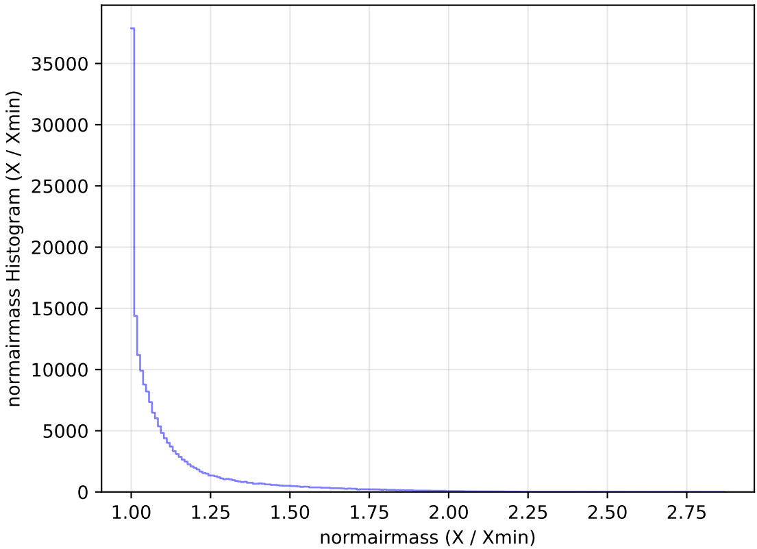
baseline_v3.3_10yrs All sky g band: normairmass Histogram
