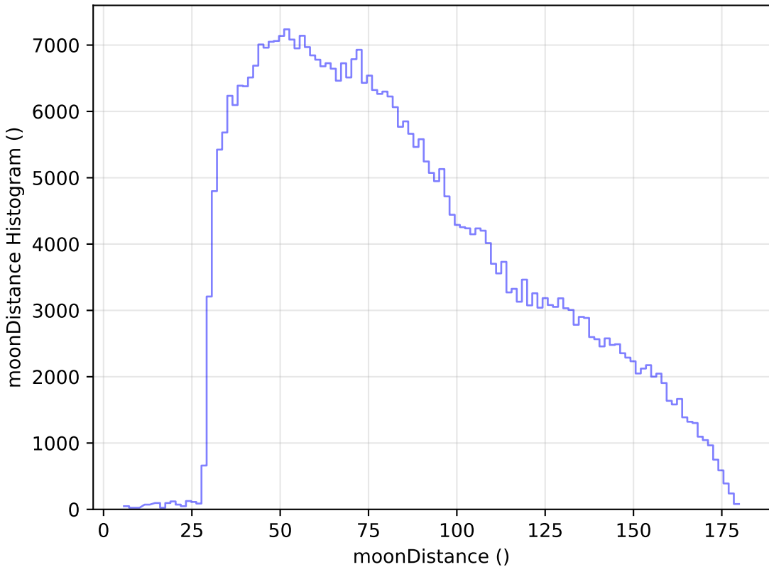
baseline_v3.3_10yrs WFD z band: moonDistance Histogram
