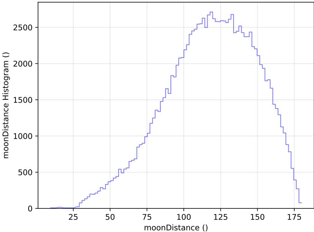
baseline_v3.3_10yrs WFD u band: moonDistance Histogram
