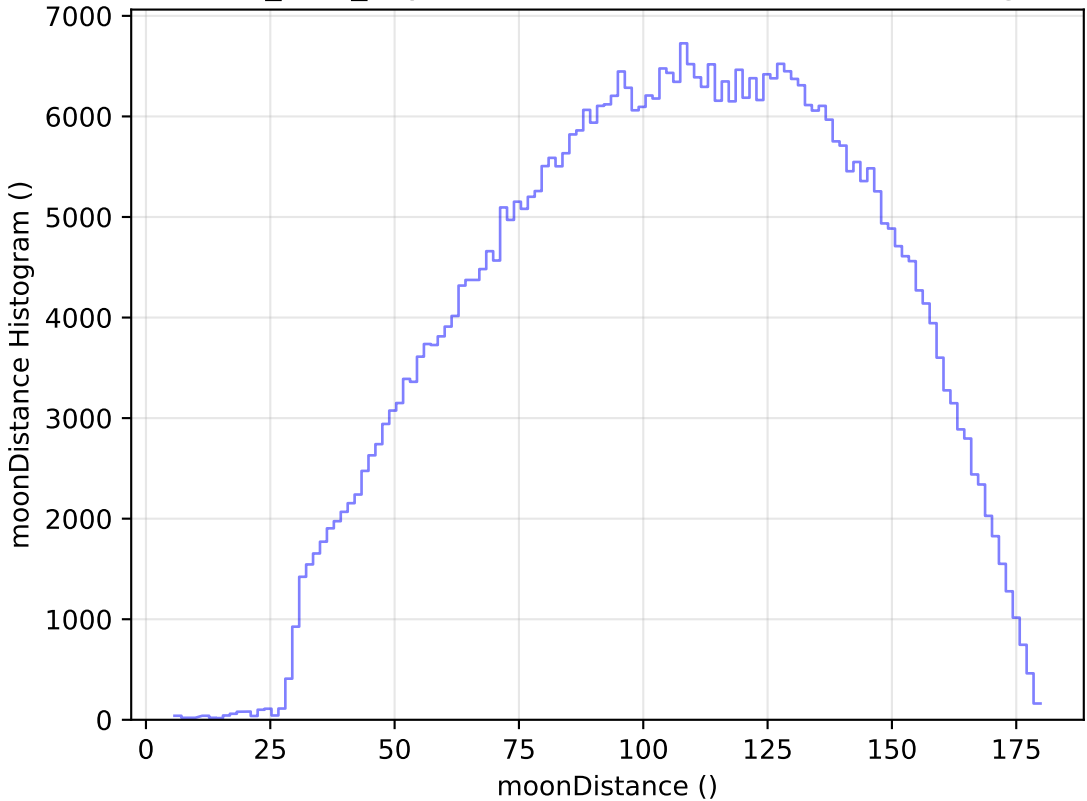
baseline_v3.3_10yrs WFD r band: moonDistance Histogram
