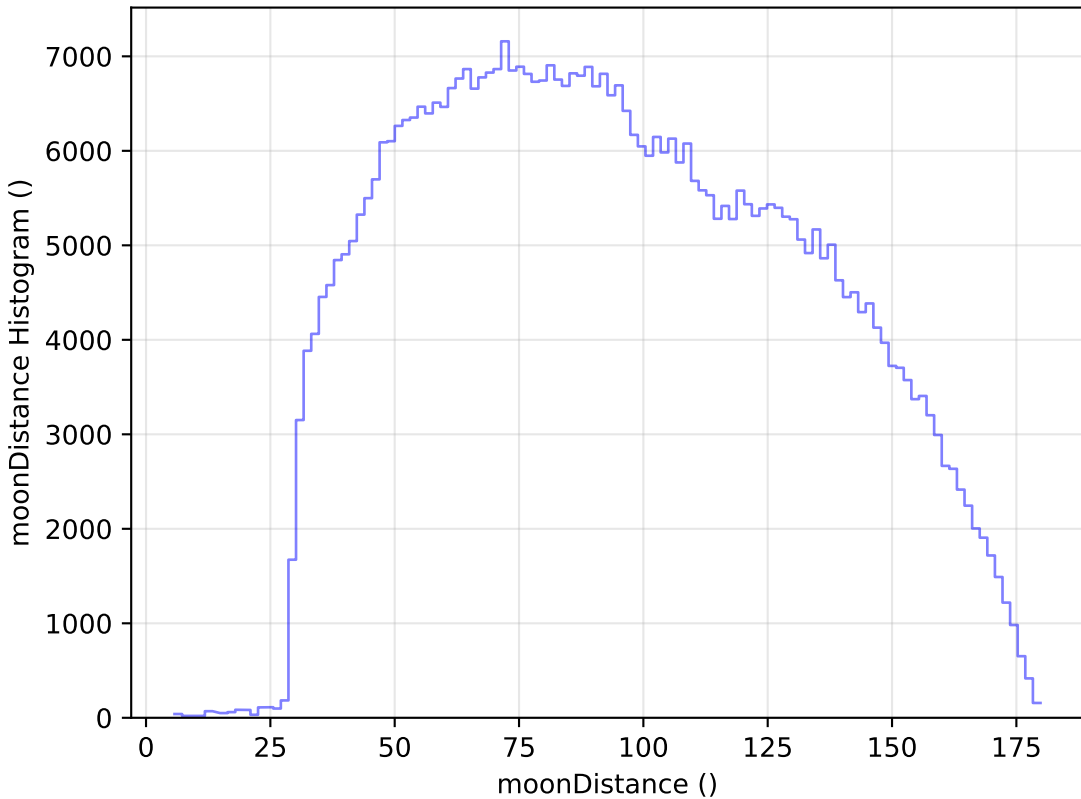
baseline_v3.3_10yrs WFD i band: moonDistance Histogram
