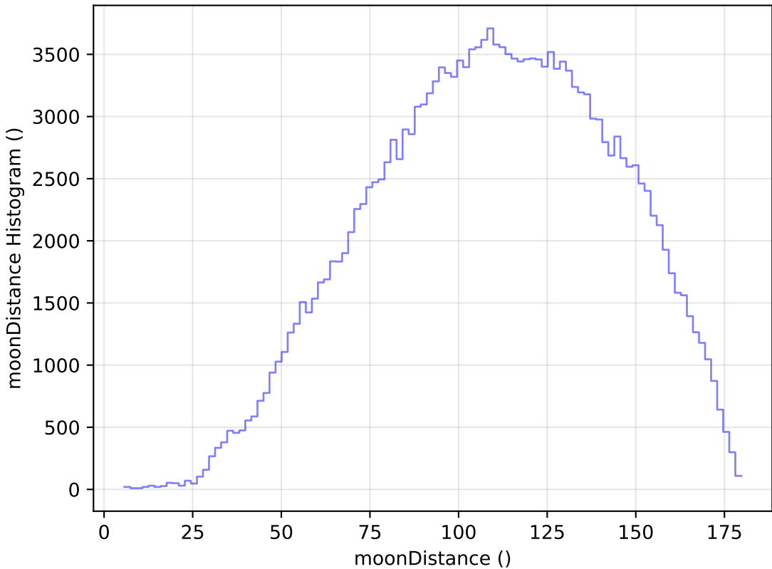
baseline_v3.3_10yrs WFD g band: moonDistance Histogram
