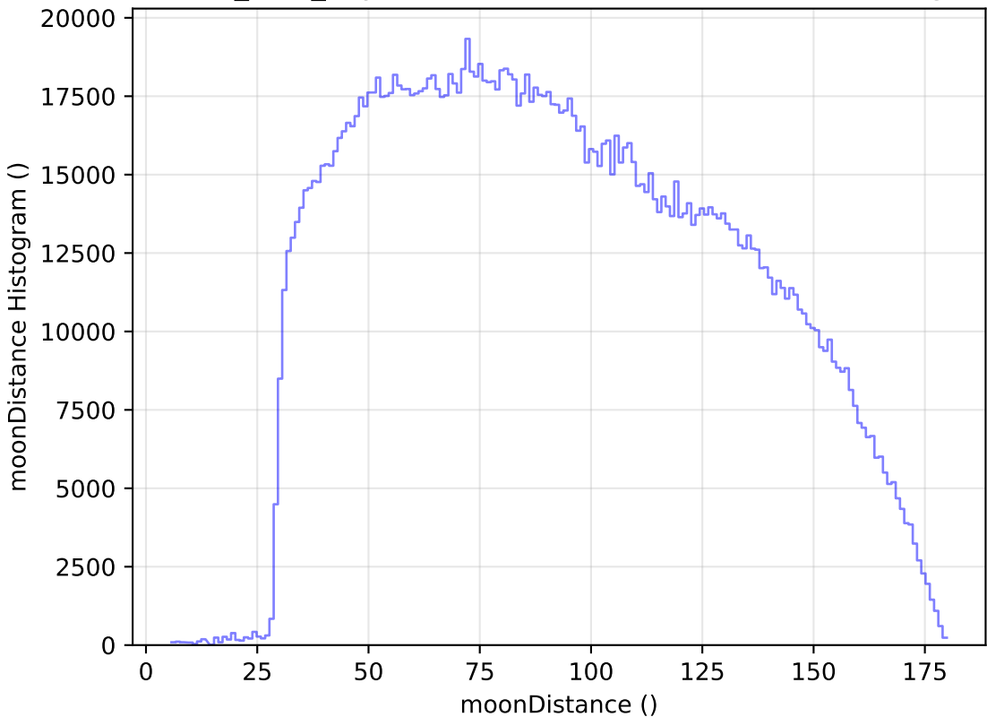
baseline_v3.3_10yrs WFD all bands: moonDistance Histogram
