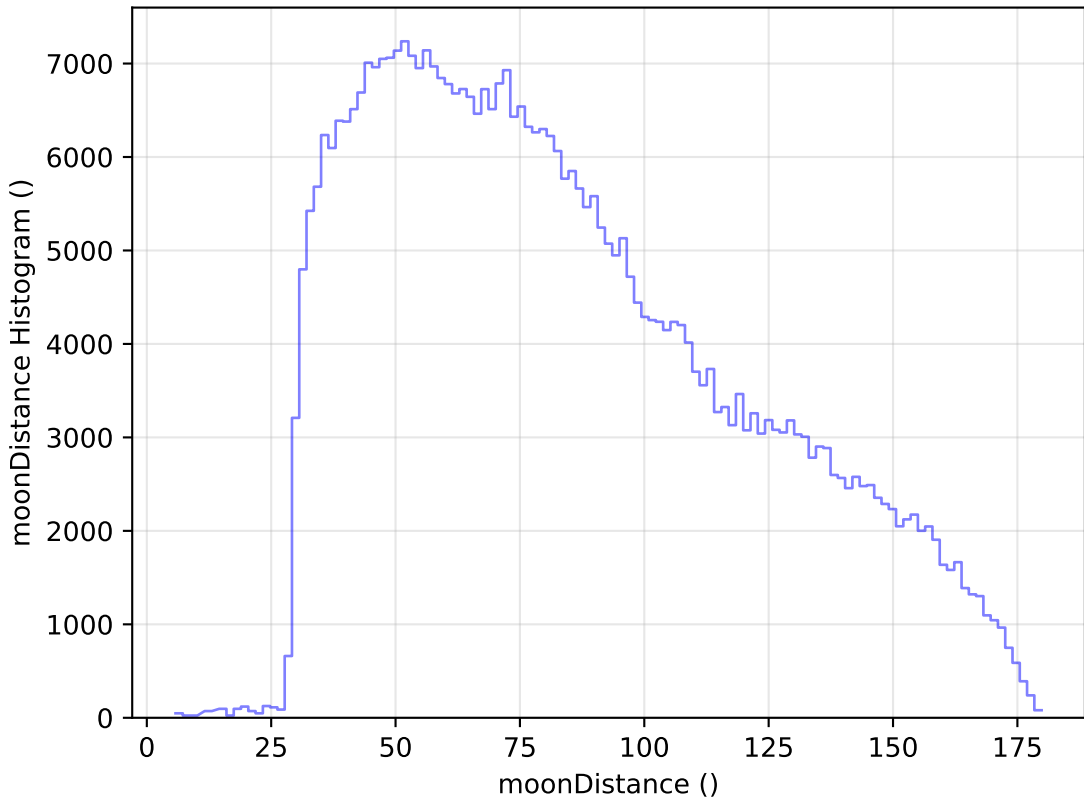
baseline_v3.3_10yrs All sky z band: moonDistance Histogram
