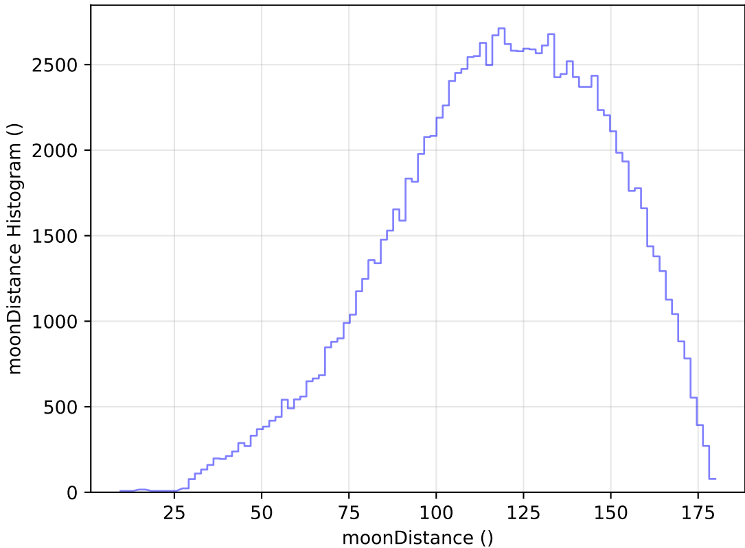
baseline_v3.3_10yrs All sky u band: moonDistance Histogram
