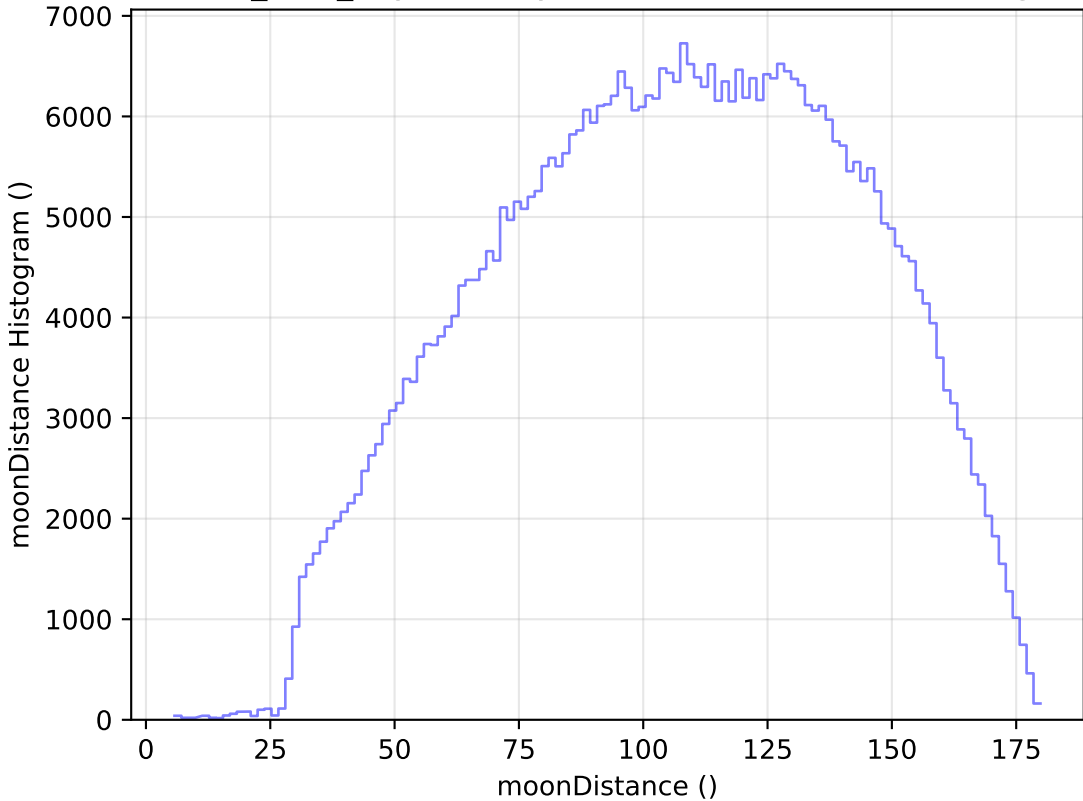
baseline_v3.3_10yrs All sky r band: moonDistance Histogram
