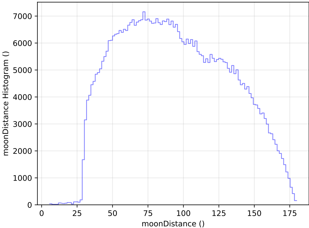
baseline_v3.3_10yrs All sky i band: moonDistance Histogram
