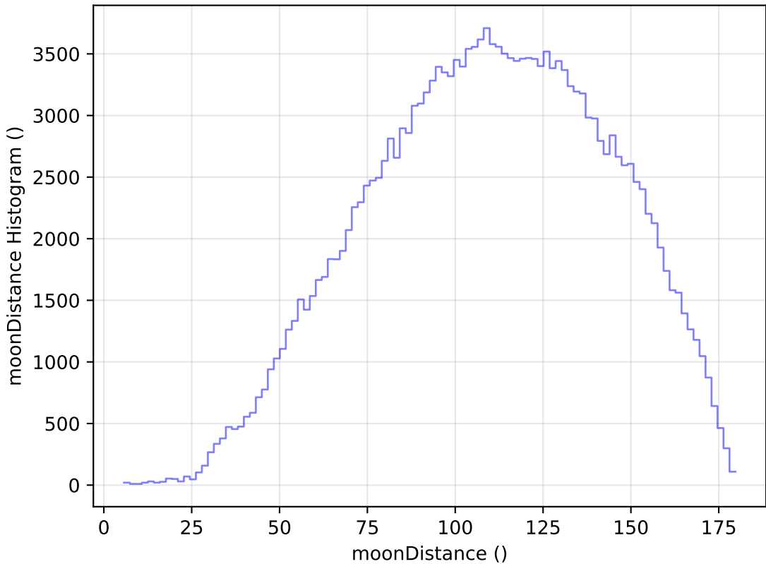
baseline_v3.3_10yrs All sky g band: moonDistance Histogram
