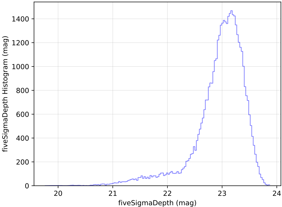
baseline_v3.3_10yrs Yr 1 z band: fiveSigmaDepth Histogram
